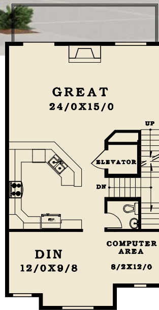
2ND FLOOR
