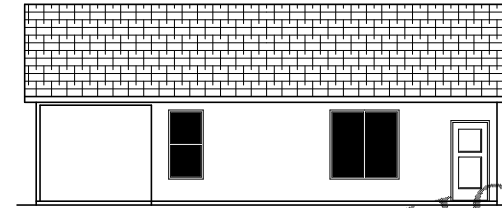
RIGHT SIDE ELEVATION SCALE 1/8"=1'-0"
