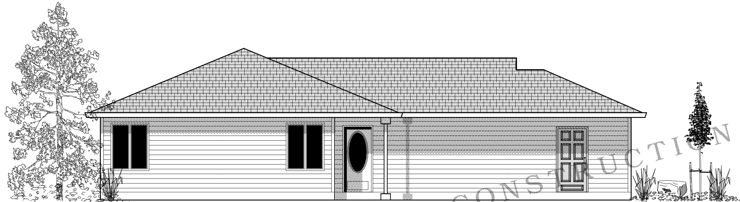
FRONT ELEVATION SCALE 1/4"=1'0"
