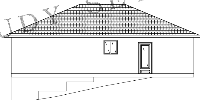
LEFT SIDE ELEVATION SCALE 1/8"=1'0"
