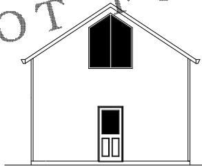
REAR ELEVATION SCALE 1/8"=1'-0"
