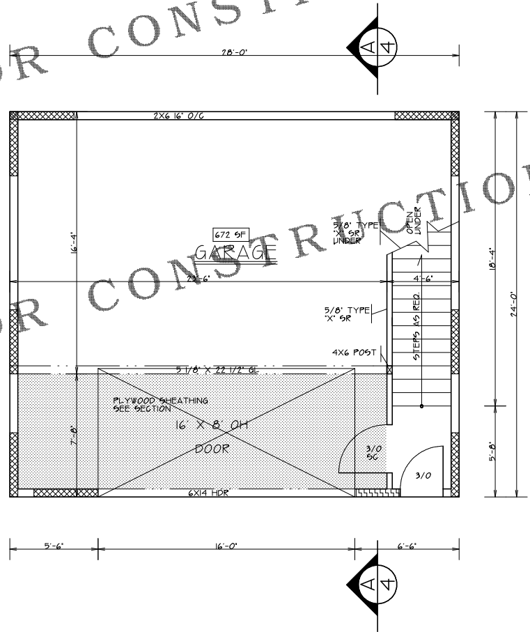
FLOOR PLAN SCALE 1/4"=1'-0"
