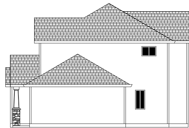
RIGHT SIDE ELEVATION SCALE 1/8"=1'0"
