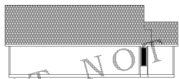
LEFT SIDE ELEVATION SCALE 1/8"=1'-0"
